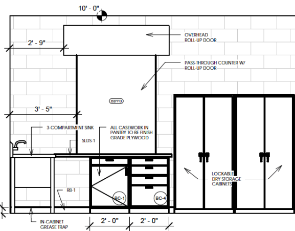
A2 PANTRY B 3/8" = 1'-0"
