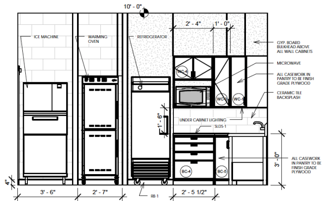
A6 PANTRY D 3/8" = 1'-0"
