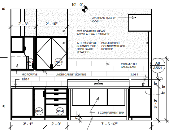
A1 PANTRY A 3/8" = 1'-0"
